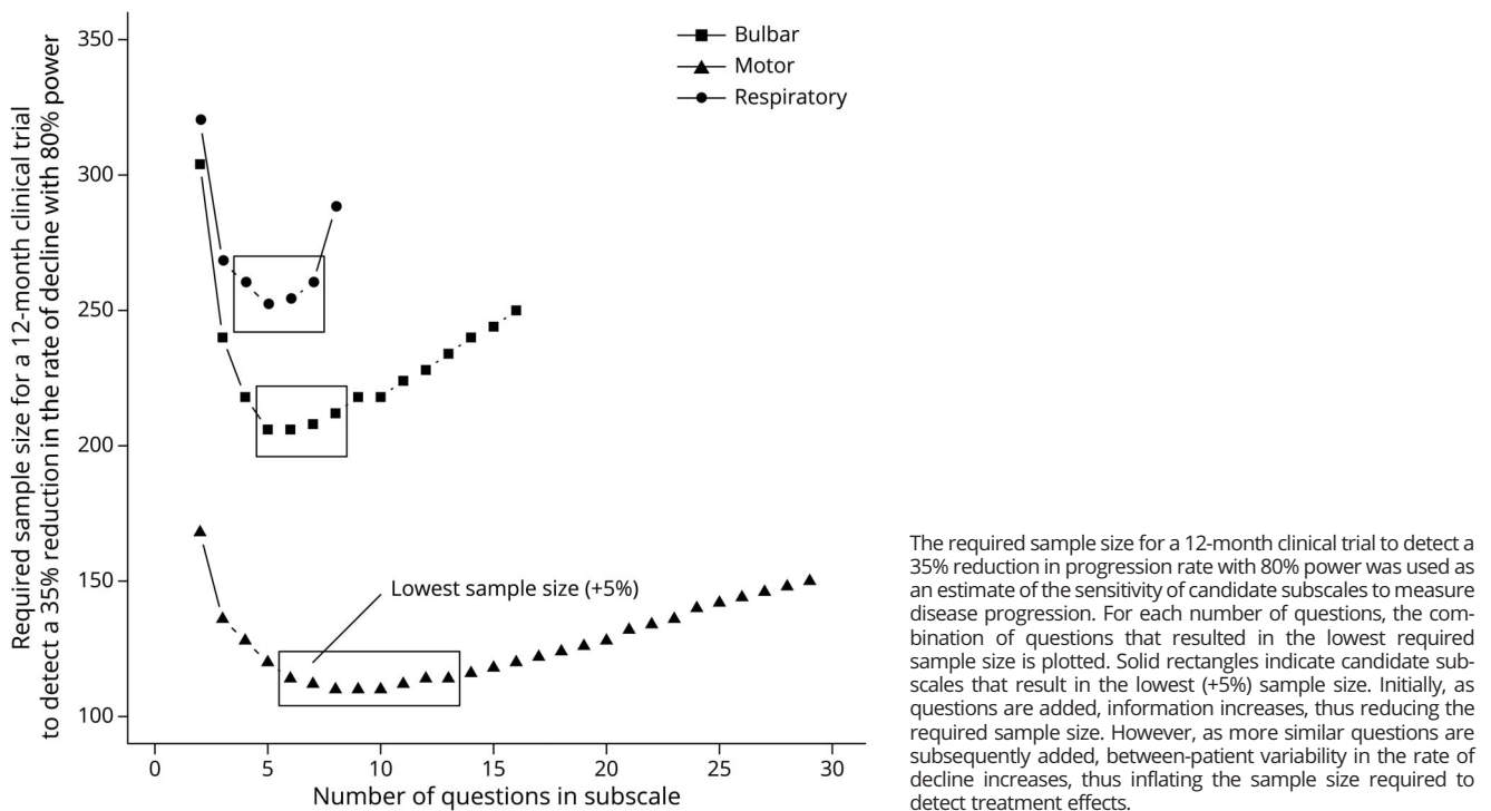
Figure 2 Number of Questions vs Required Sample Size per Subscale
